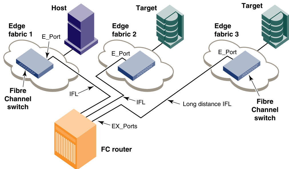
FIGURE 72 A metaSAN with inter-fabric links
