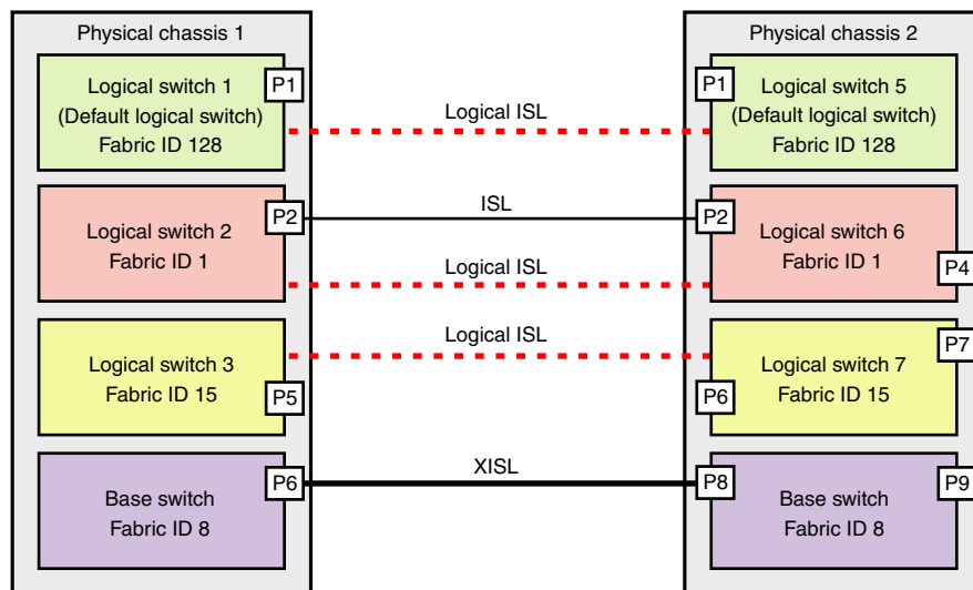
FIGURE 27 Logical fabric using ISLs and XISLs
