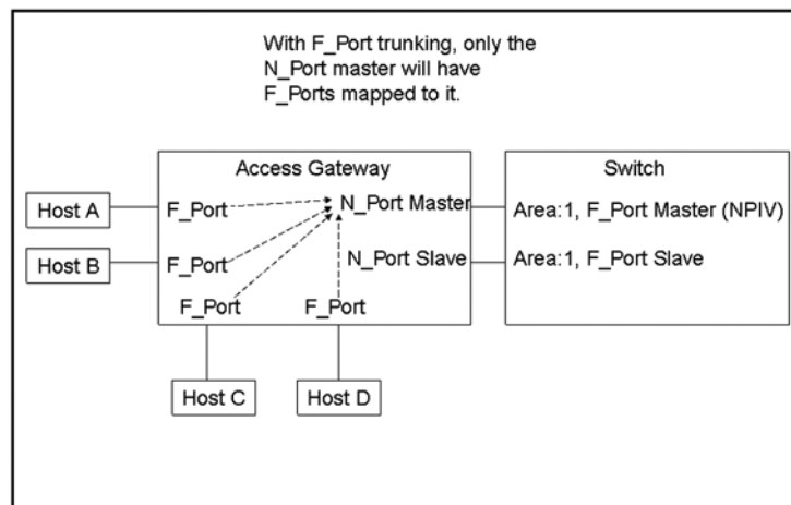
FIGURE 71 Switch in Access Gateway mode with F_Port masterless trunking
