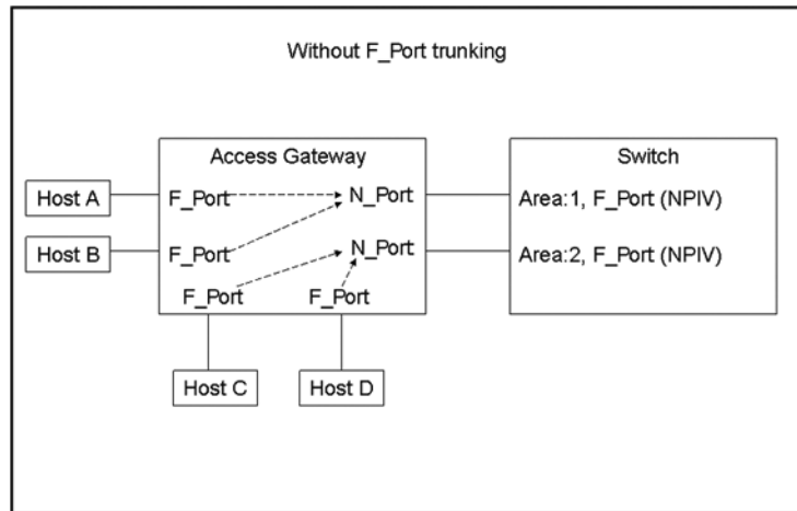
FIGURE 70 Switch in Access Gateway mode without F_Port trunking
