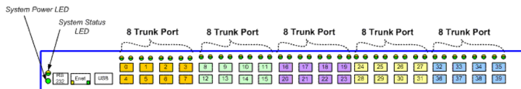
FIGURE 69 Trunk group configuration for the Brocade 5100
