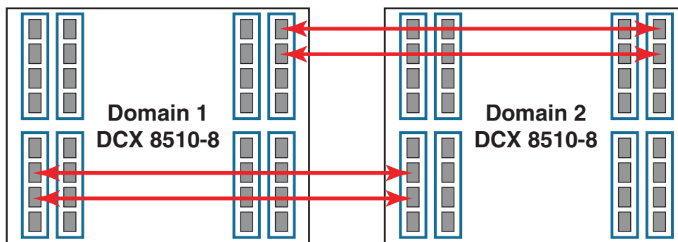
FIGURE 58 Minimum configuration for 64 Gbps ICLs
