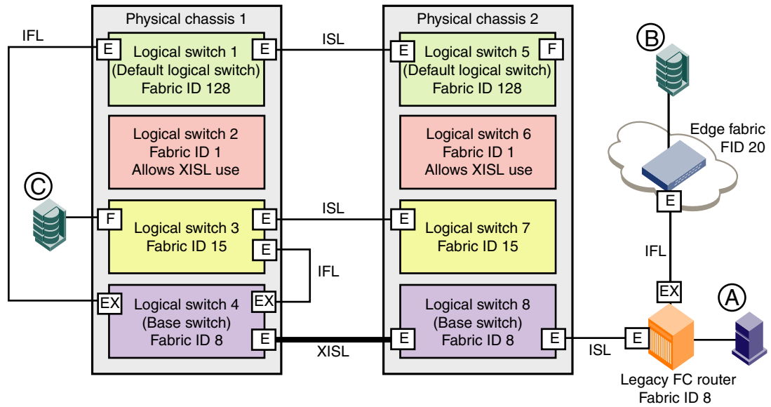
FIGURE 82 Backbone-to-edge routing across base switch using FC router in legacy mode
