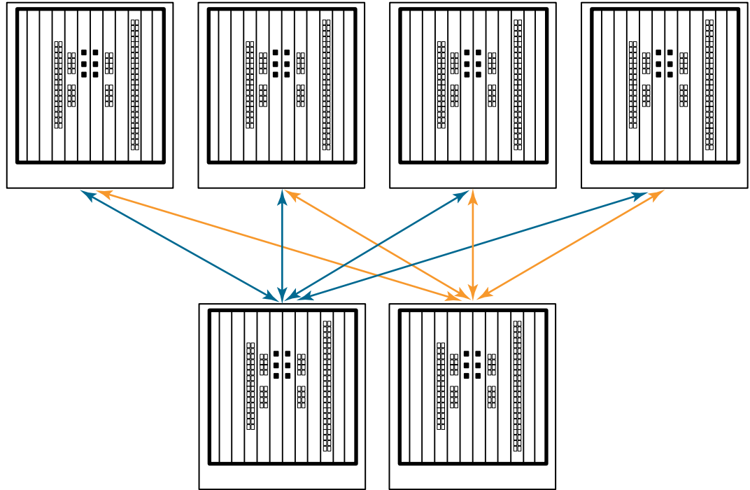
FIGURE 61 64 Gbps ICL core-edge topology
