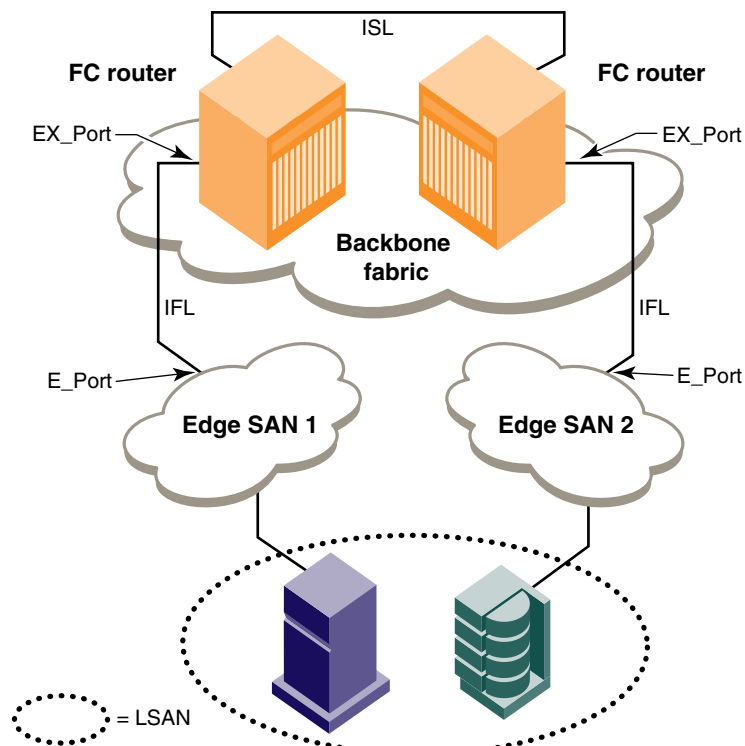
FIGURE 74 Edge SANs connected through a backbone fabric
