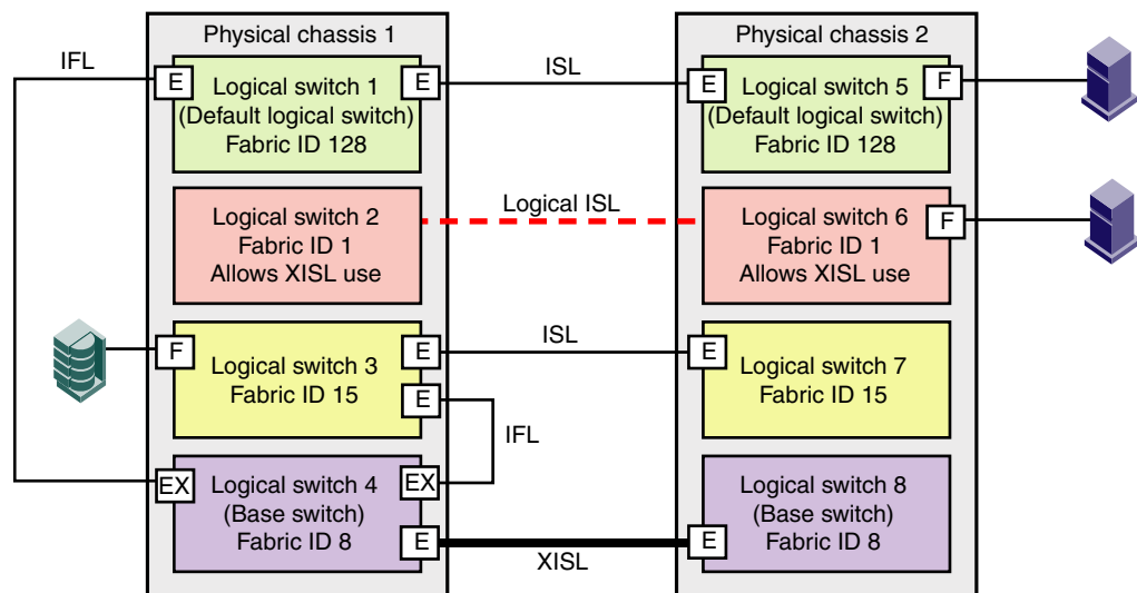
FIGURE 80 EX_Ports in a base switch
