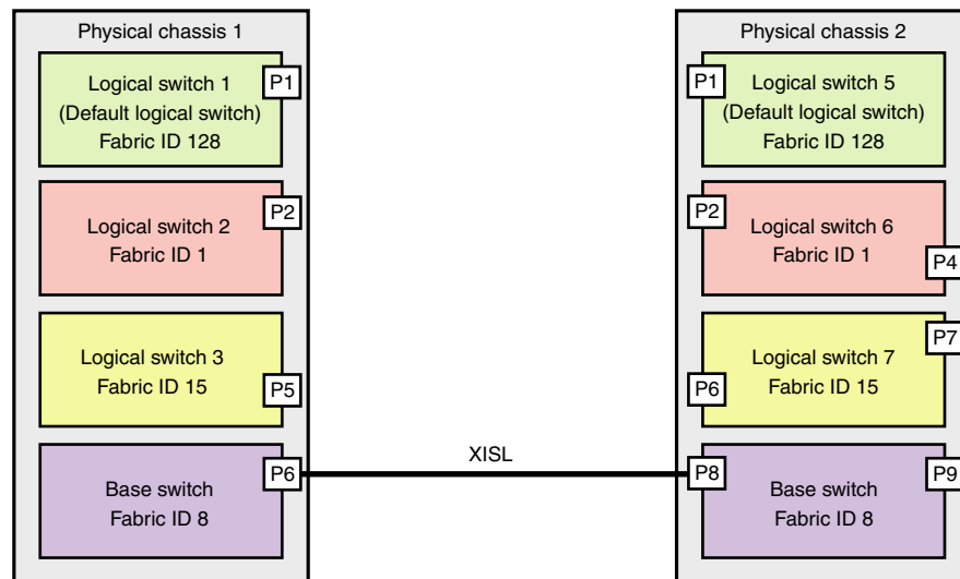
FIGURE 25 Base switches connected by an XISL
