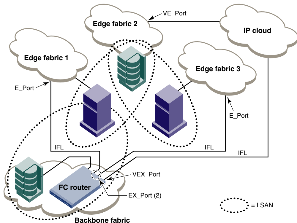
FIGURE 73 A metaSAN with edge-to-edge and backbone fabrics and LSAN zones
