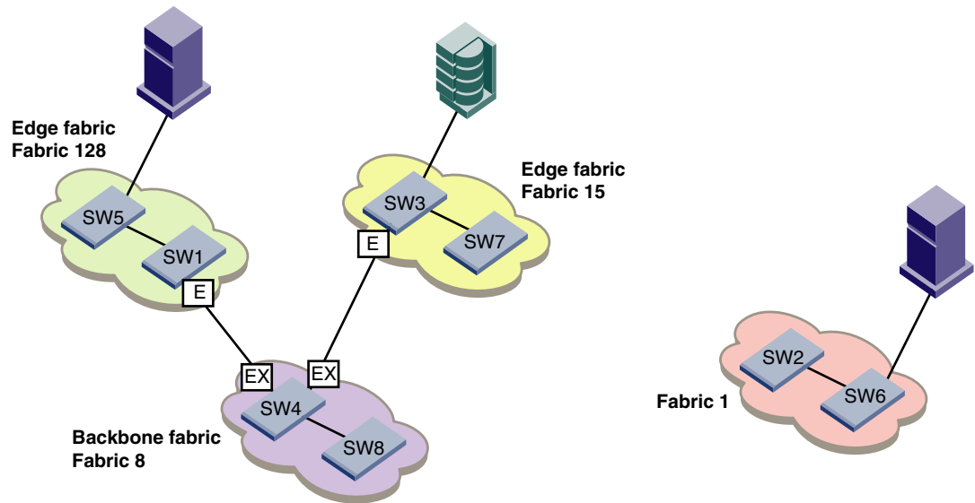
FIGURE 81 Logical representation of EX_Ports in a base switch
