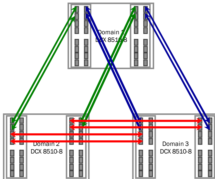
FIGURE 60 ICL triangular topology with Brocade DCX 8510-8 chassis
