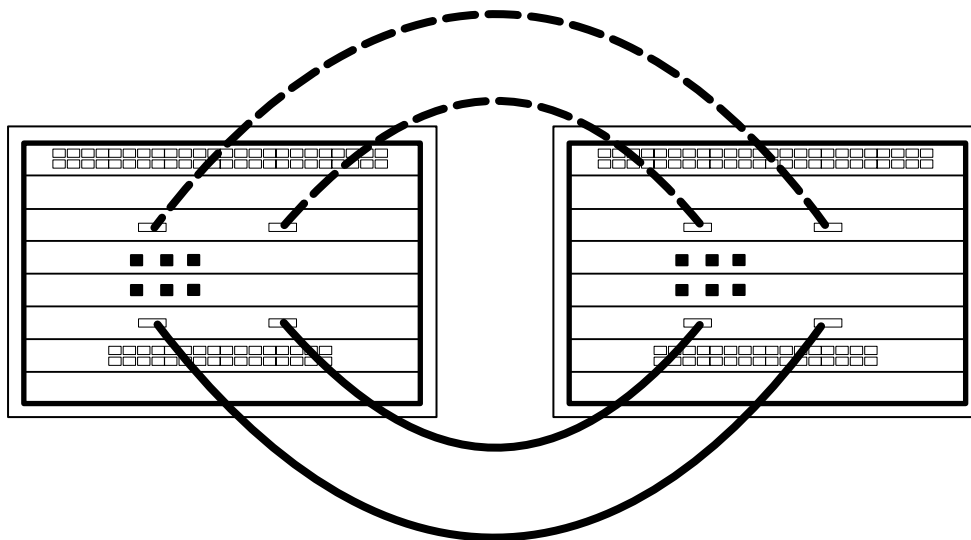
FIGURE 59 DCX-4S allowed ICL connections
