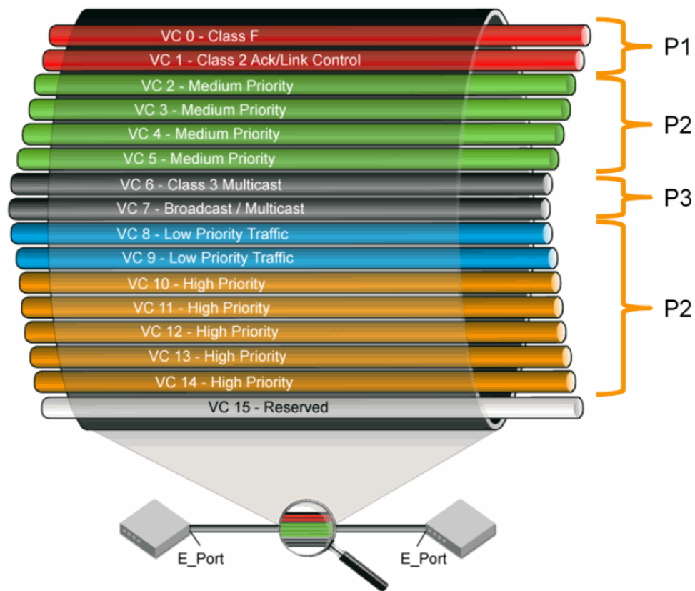
FIGURE 7 Virtual channels on a QoS-enabled ISL
